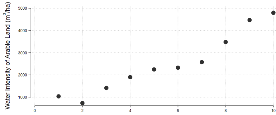
(b) Deciles of Groundwater Access (→ Higher Water Table)
