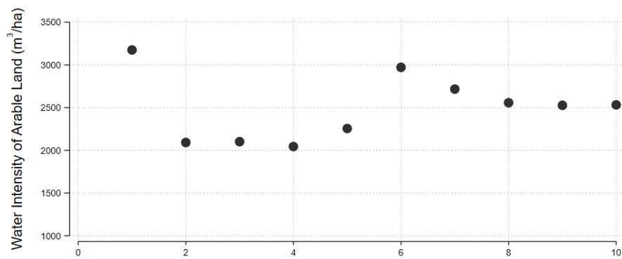
(c) Deciles of Trends in Total Water Storage (→ Gaining More Water)
