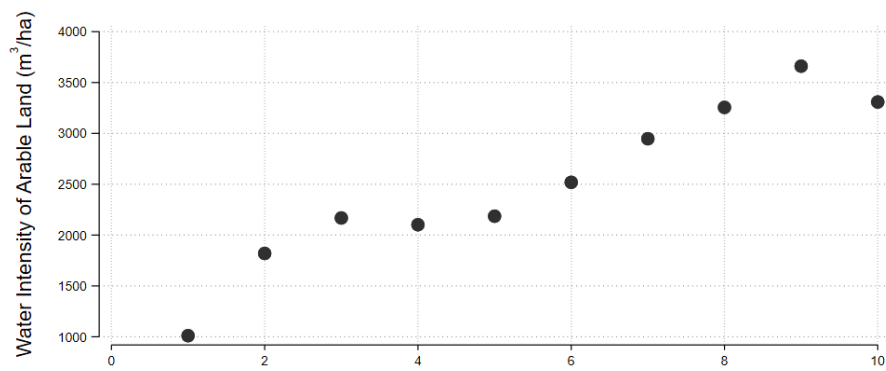
(c) Deciles of Trends in Total Water Storage (→ Gaining More Water)
